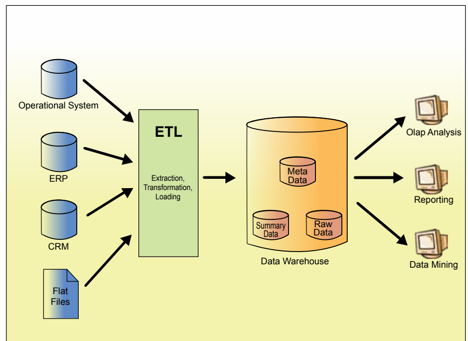
A typical Data Warehouse view
